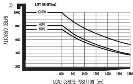
RATED CAPACITIES AND LOAD CENTERS GRAPH
